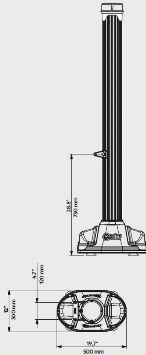
SIDE VIEW
